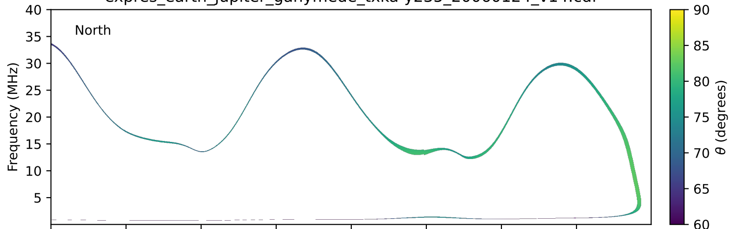
expres_earth_jupiter_ganymede_txka-y235_20060124_v14.cdf
