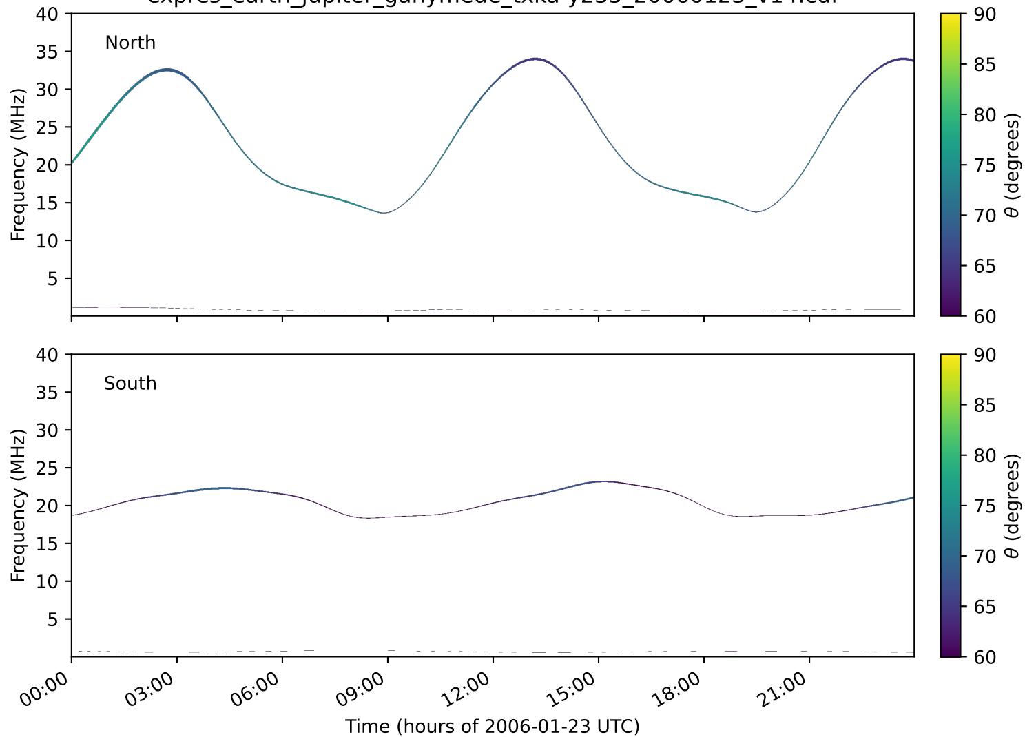
expres_earth_jupiter_ganymede_txka-y235_20060123_v14.cdf
