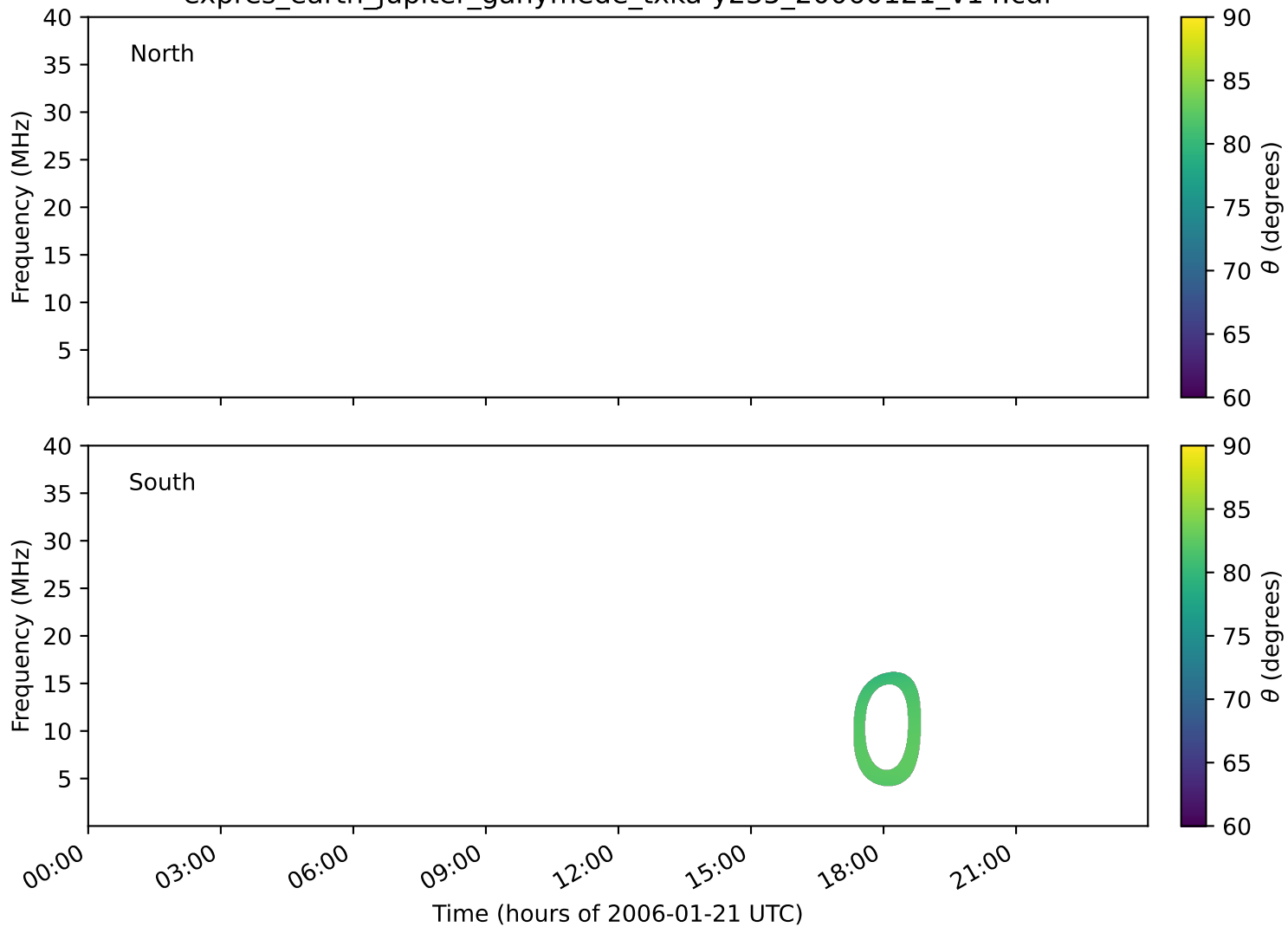
expres_earth_jupiter_ganymede_txka-y235_20060121_v14.cdf
