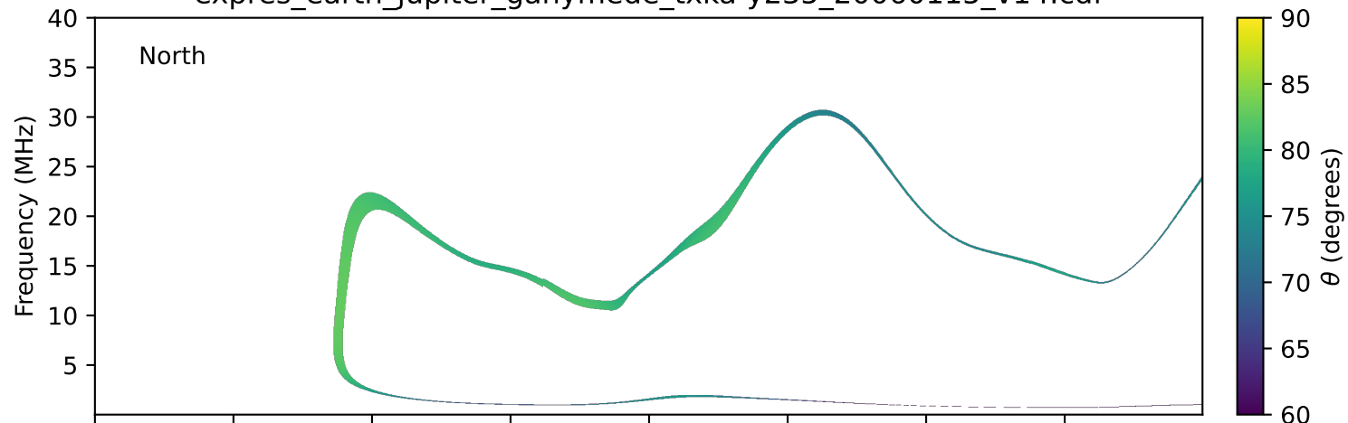
expres_earth_jupiter_ganymede_txka-y235_20060115_v14.cdf
