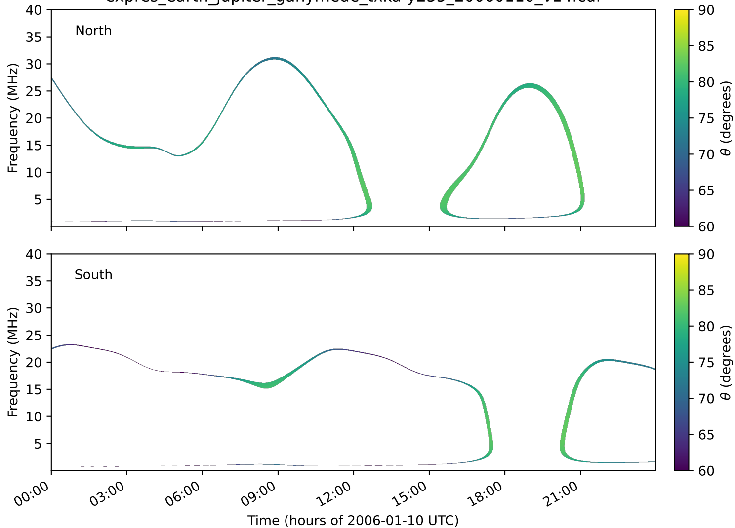
expres_earth_jupiter_ganymede_txka-y235_20060110_v14.cdf
