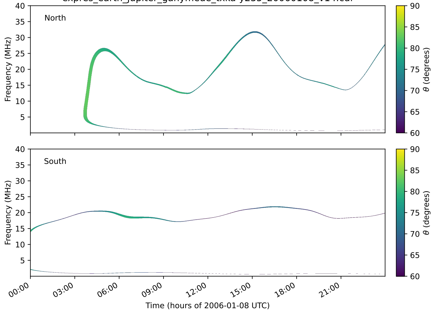
expres_earth_jupiter_ganymede_txka-y235_20060108_v14.cdf
