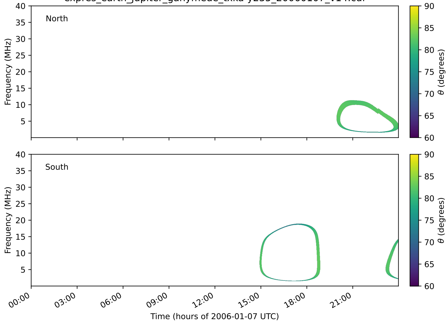
expres_earth_jupiter_ganymede_txka-y235_20060107_v14.cdf
