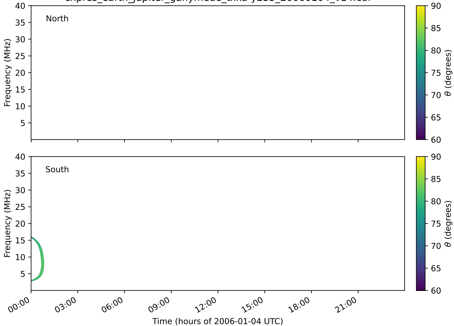
expres_earth_jupiter_ganymede_txka-y235_20060104_v14.cdf
