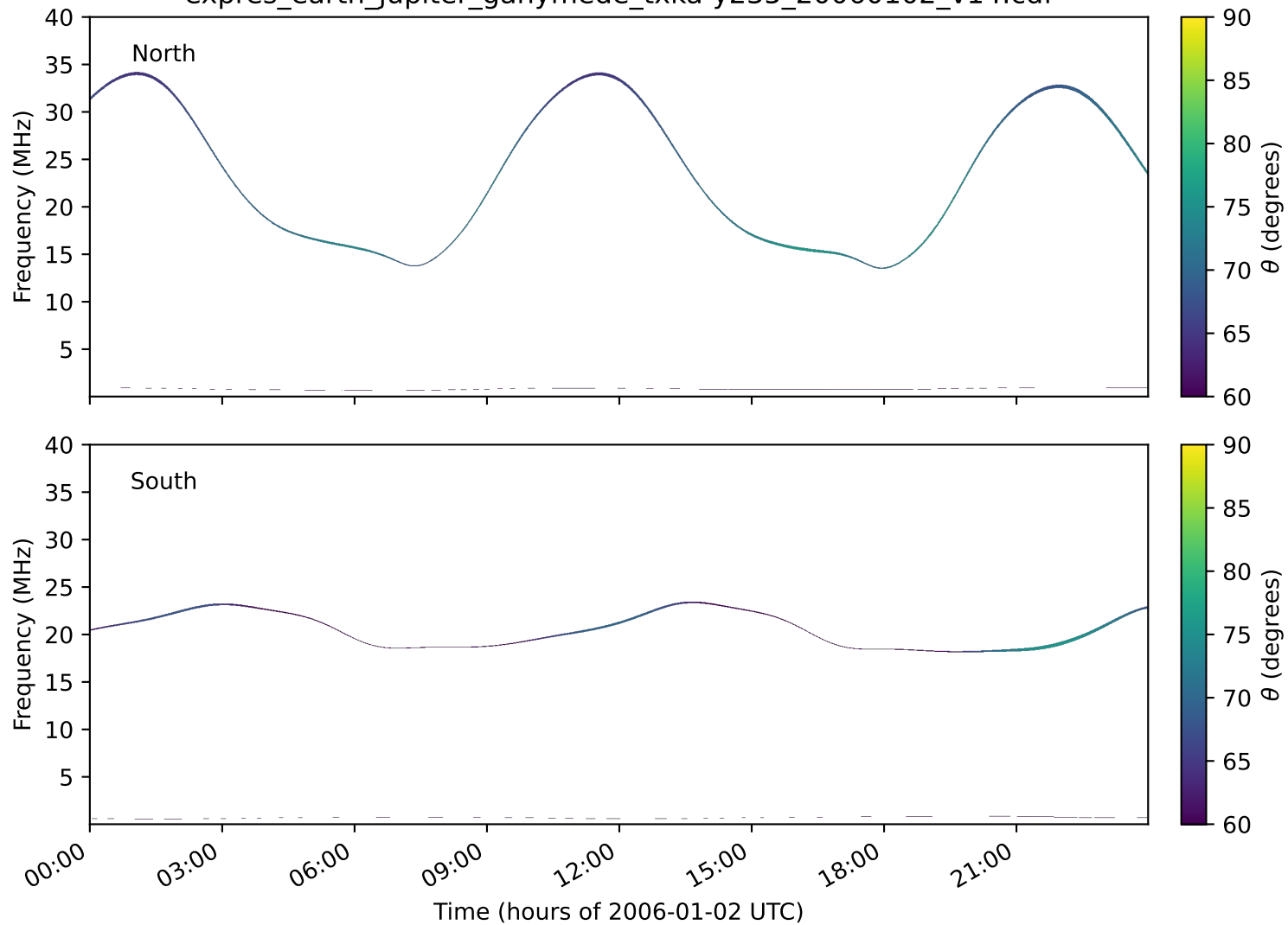
expres_earth_jupiter_ganymede_txka-y235_20060102_v14.cdf
