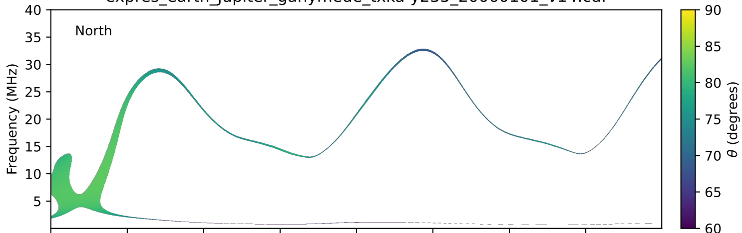
expres_earth_jupiter_ganymede_txka-y235_20060101_v14.cdf
