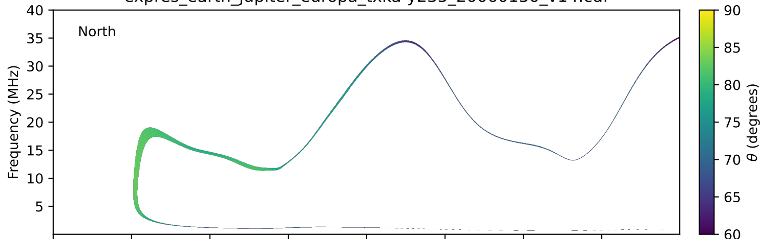
expres_earth_jupiter_europa_txka-y235_20060130_v14.cdf
