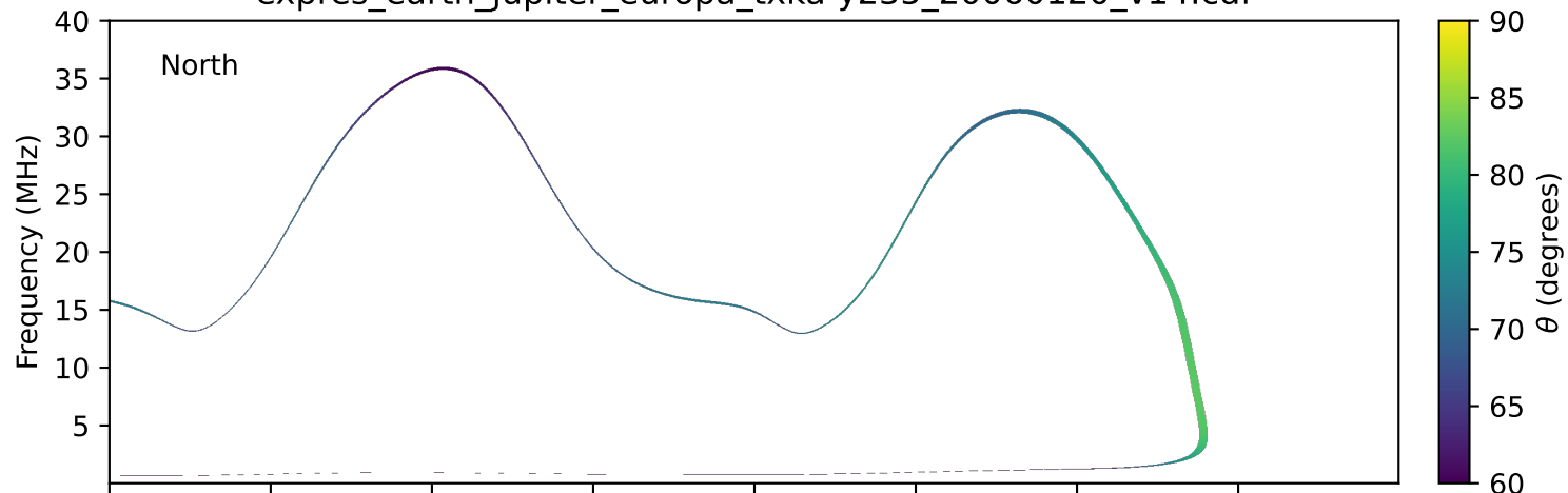
expres_earth_jupiter_europa_txka-y235_20060120_v14.cdf
