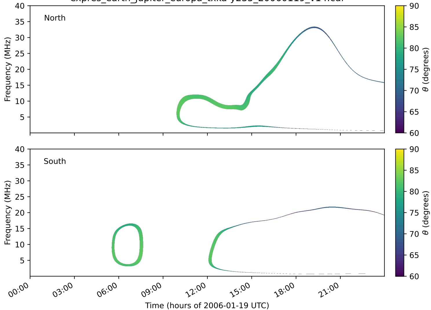
expres_earth_jupiter_europa_txka-y235_20060119_v14.cdf
