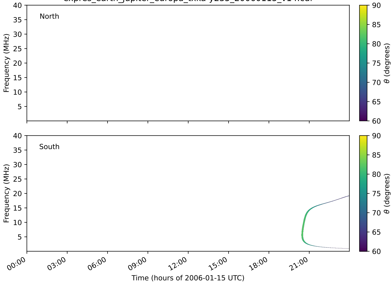
expres_earth_jupiter_europa_txka-y235_20060115_v14.cdf
