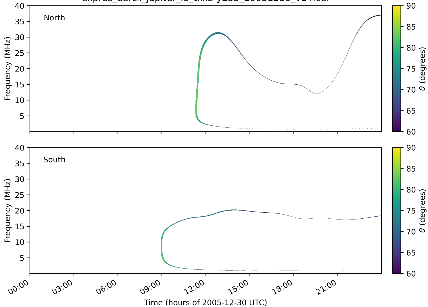
expres_earth_jupiter_io_txka-y235_20051230_v14.cdf
