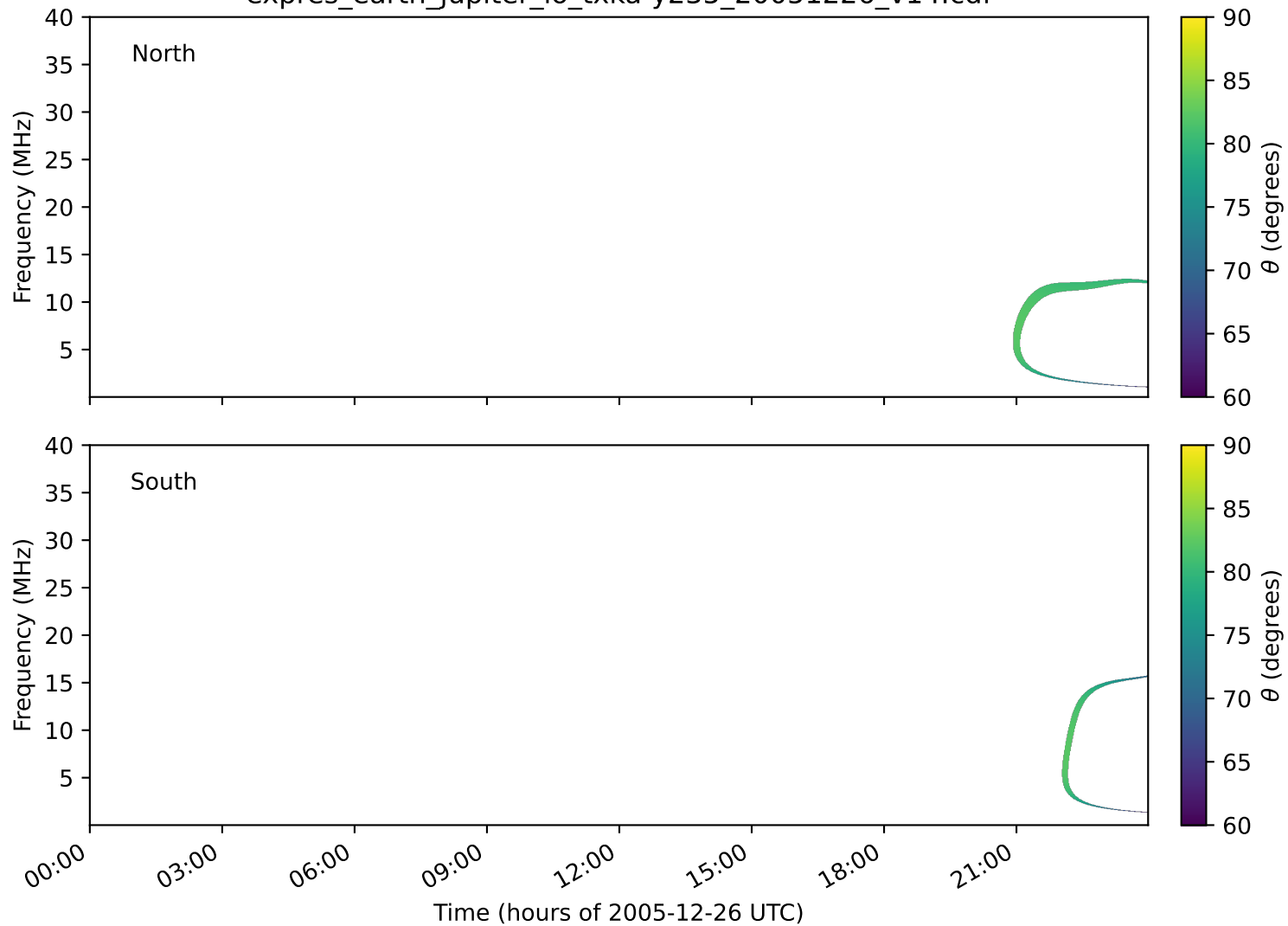
expres_earth_jupiter_io_txka-y235_20051226_v14.cdf
