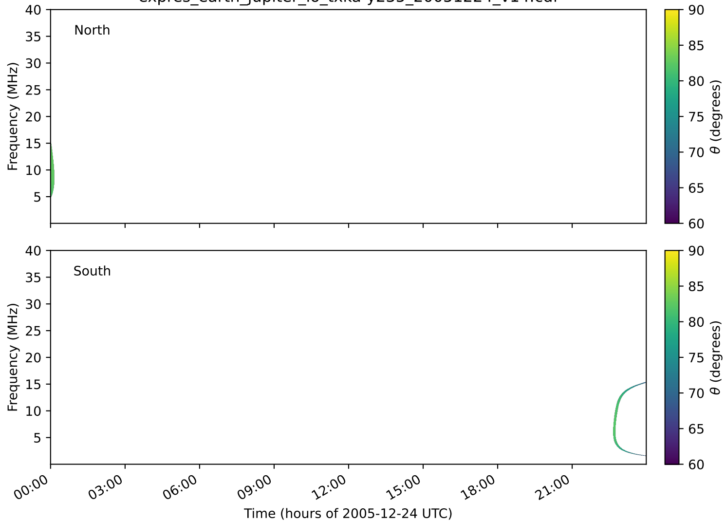
expres_earth_jupiter_io_txka-y235_20051224_v14.cdf
