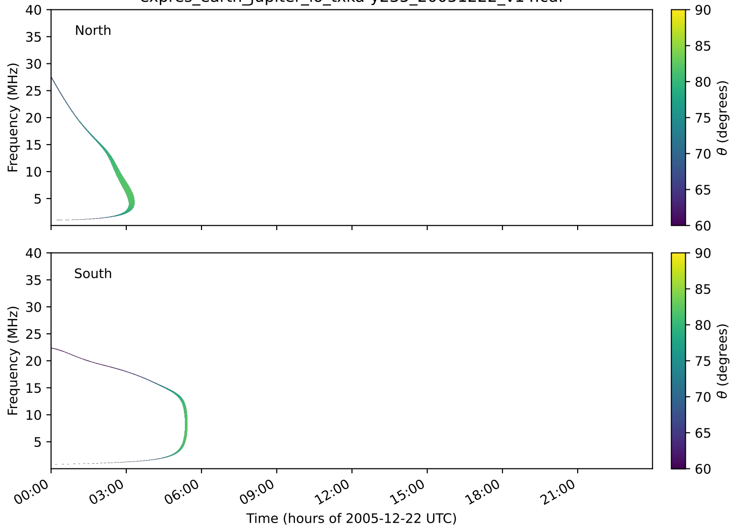
expres_earth_jupiter_io_txka-y235_20051222_v14.cdf
