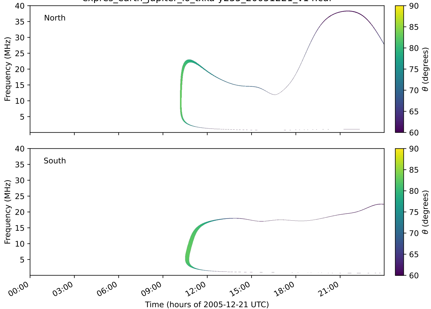
expres_earth_jupiter_io_txka-y235_20051221_v14.cdf
