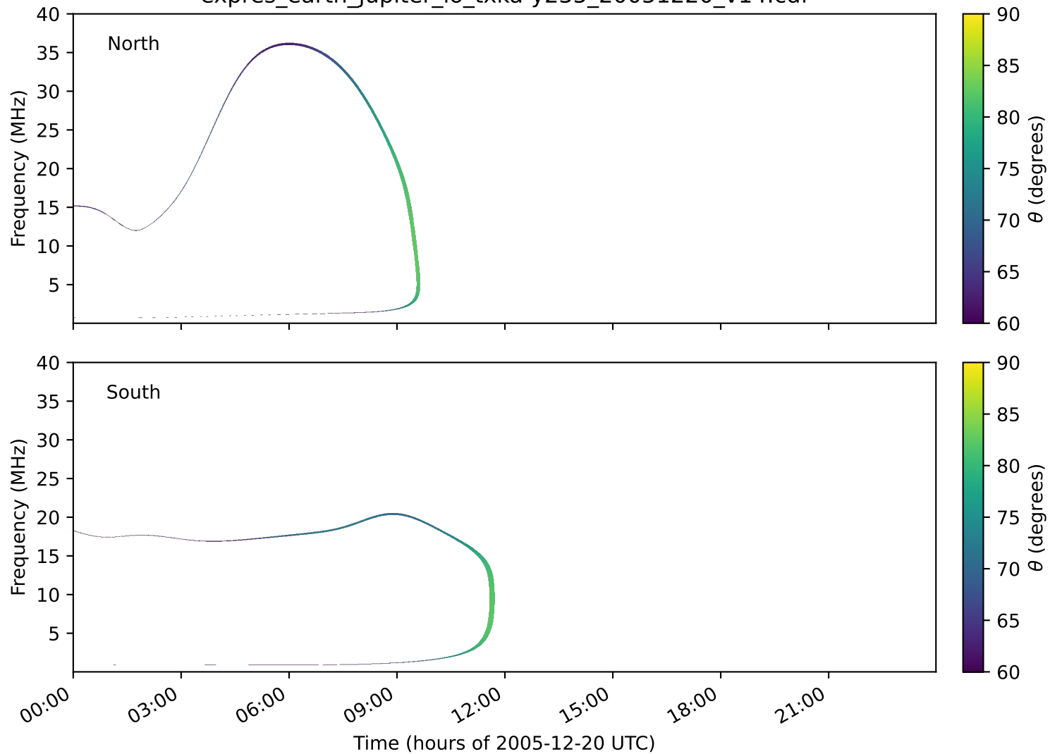
expres_earth_jupiter_io_txka-y235_20051220_v14.cdf
