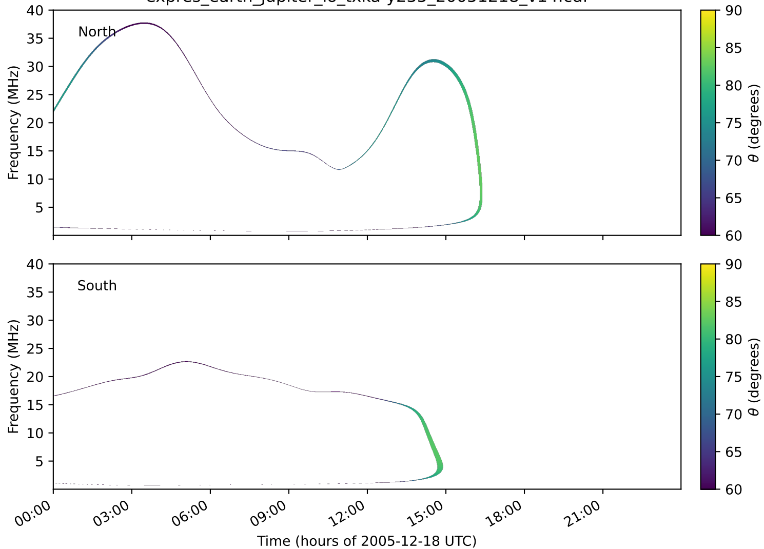
expres_earth_jupiter_io_txka-y235_20051218_v14.cdf
