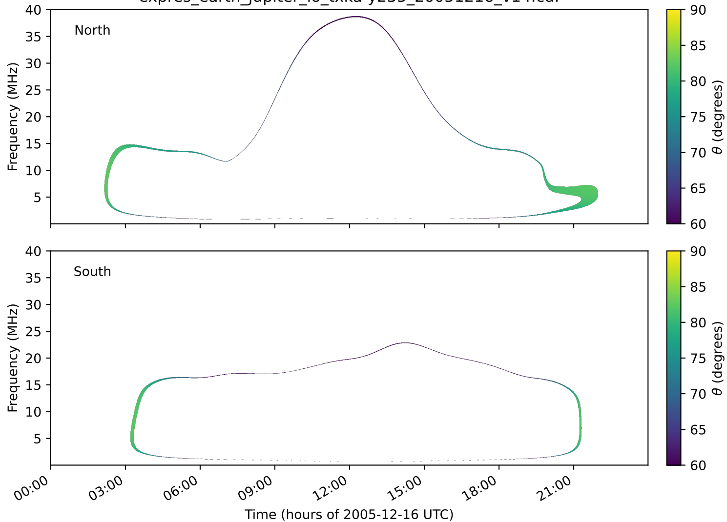
expres_earth_jupiter_io_txka-y235_20051216_v14.cdf
