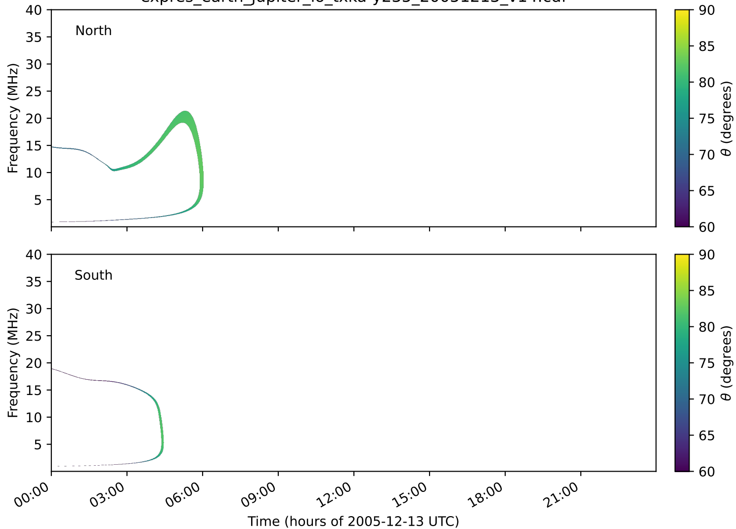
expres_earth_jupiter_io_txka-y235_20051213_v14.cdf
