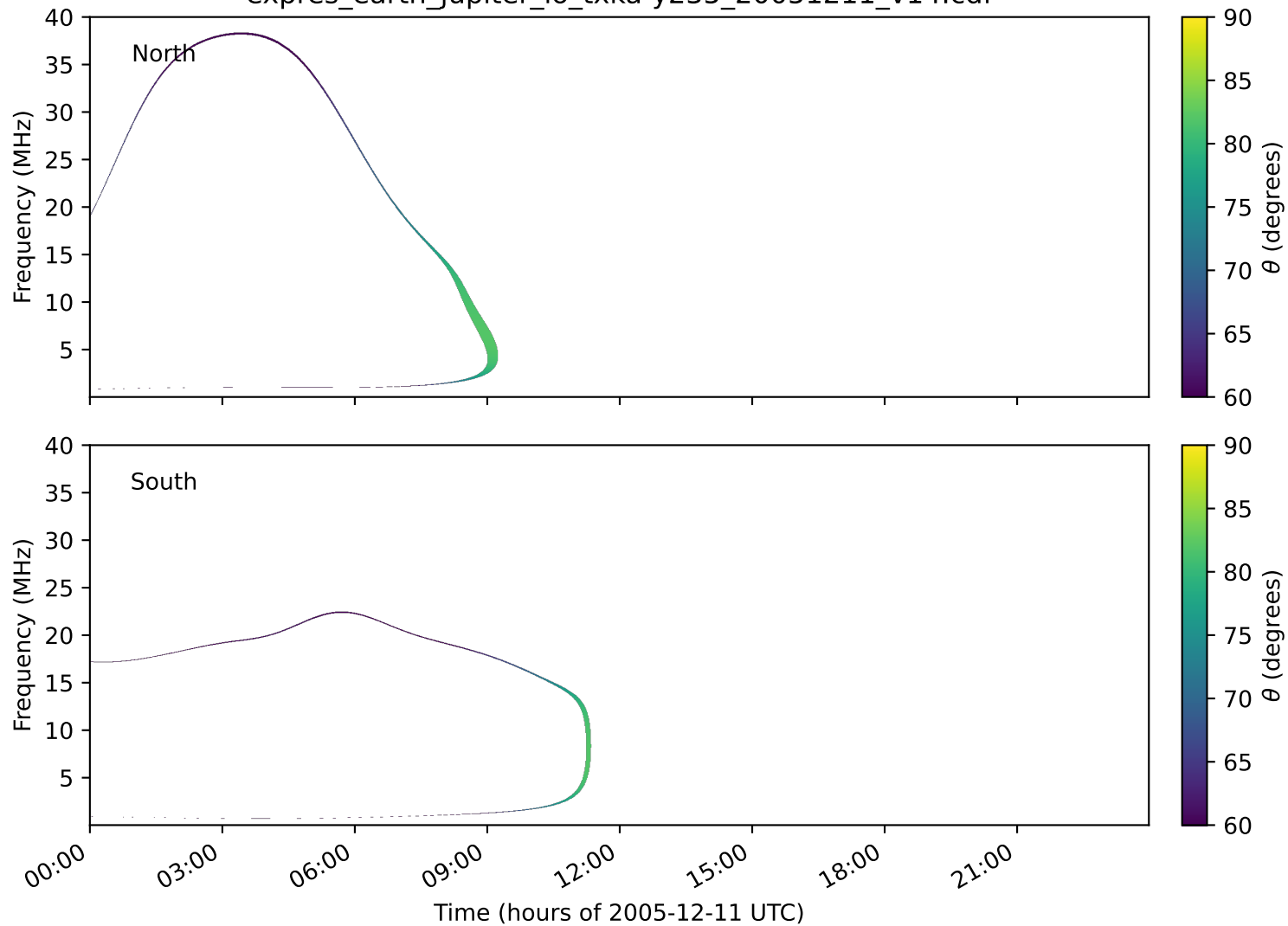
expres_earth_jupiter_io_txka-y235_20051211_v14.cdf
