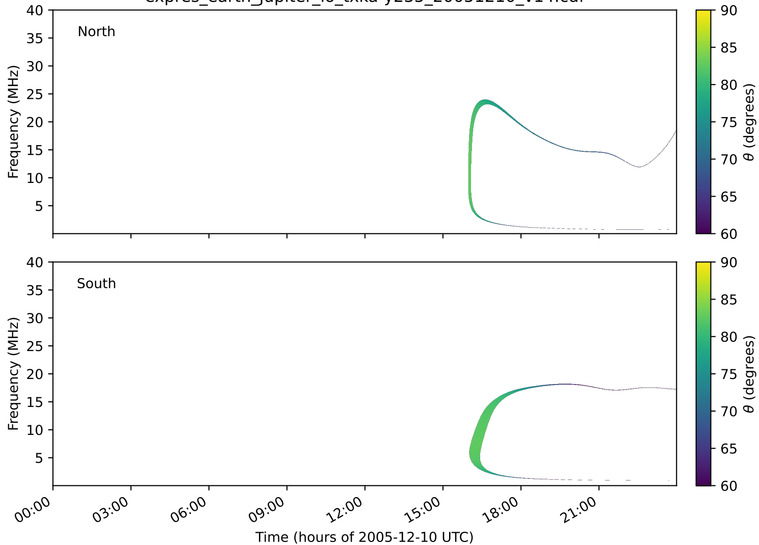
expres_earth_jupiter_io_txka-y235_20051210_v14.cdf
