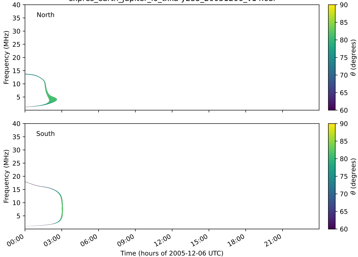
expres_earth_jupiter_io_txka-y235_20051206_v14.cdf
