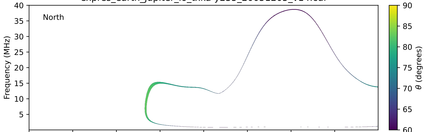
expres_earth_jupiter_io_txka-y235_20051205_v14.cdf
