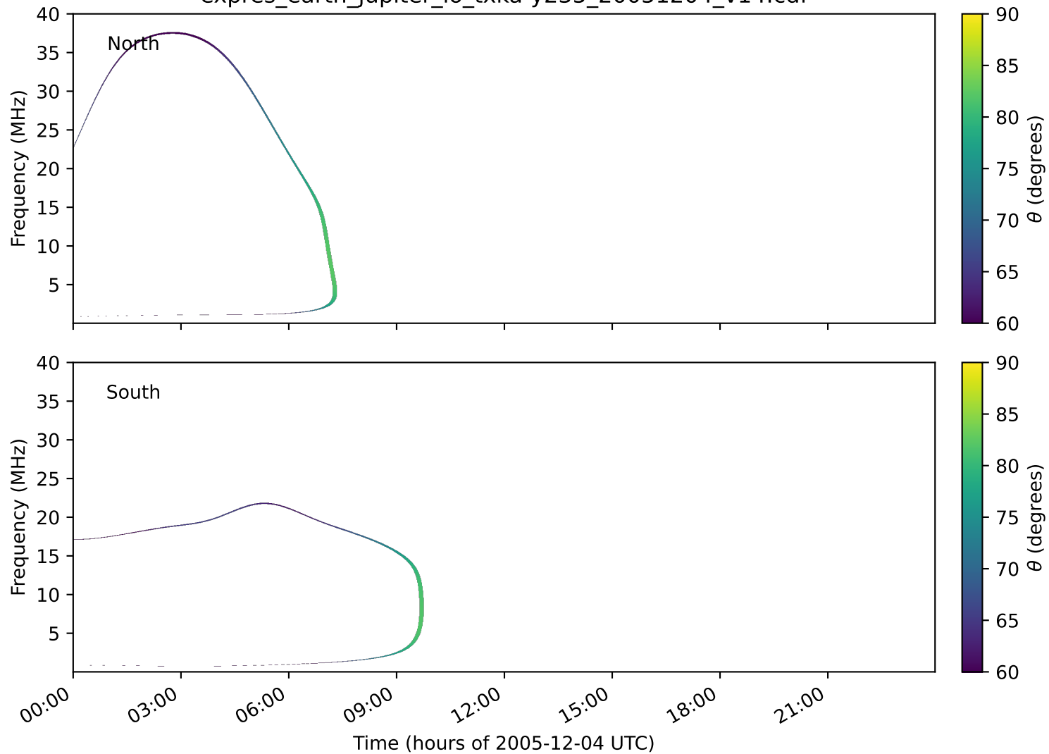
expres_earth_jupiter_io_txka-y235_20051204_v14.cdf
