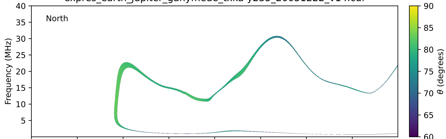
expres_earth_jupiter_ganymede_txka-y235_20051222_v14.cdf
