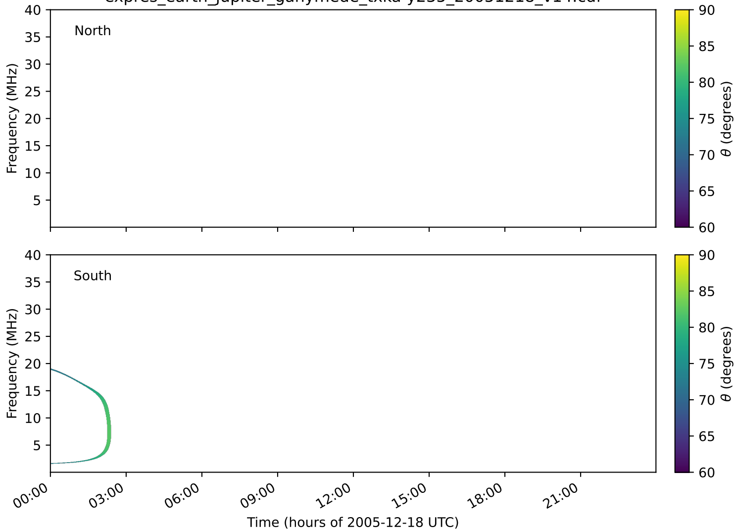
expres_earth_jupiter_ganymede_txka-y235_20051218_v14.cdf
