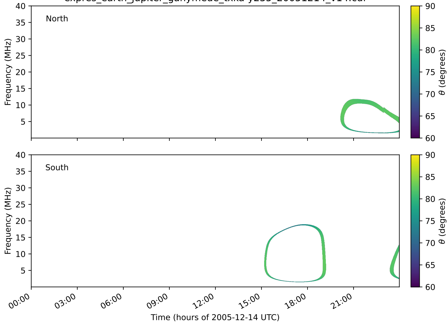
expres_earth_jupiter_ganymede_txka-y235_20051214_v14.cdf
