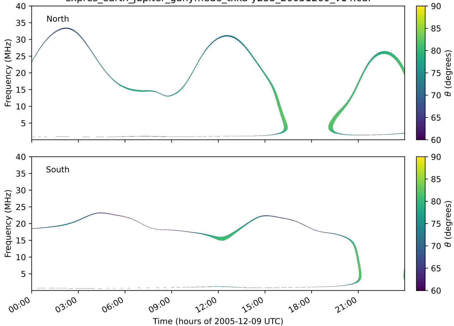
expres_earth_jupiter_ganymede_txka-y235_20051209_v14.cdf
