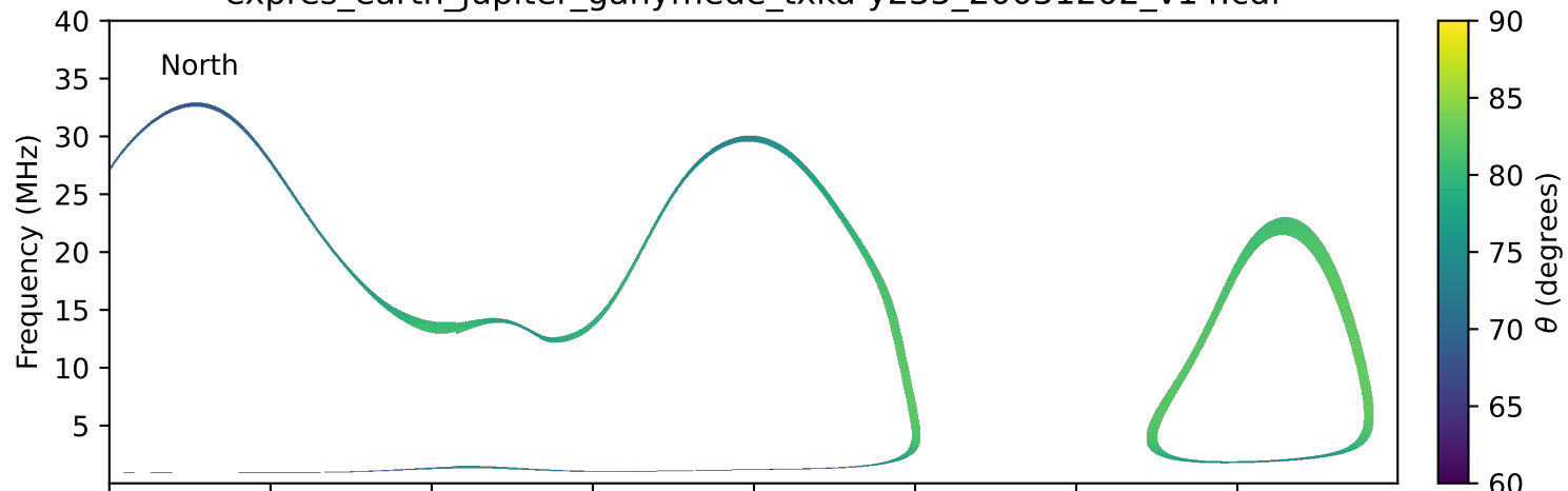
expres_earth_jupiter_ganymede_txka-y235_20051202_v14.cdf
