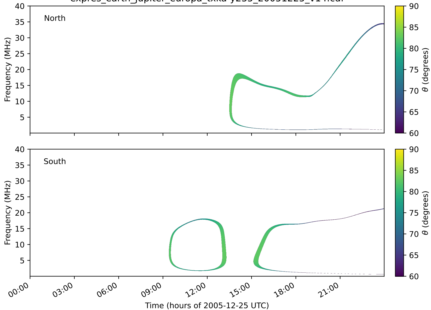
expres_earth_jupiter_europa_txka-y235_20051225_v14.cdf
