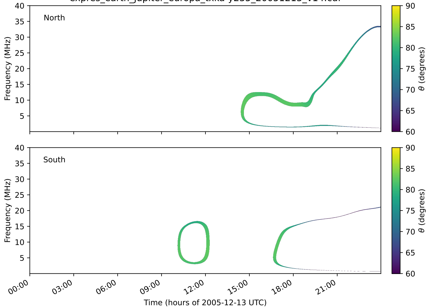
expres_earth_jupiter_europa_txka-y235_20051213_v14.cdf
