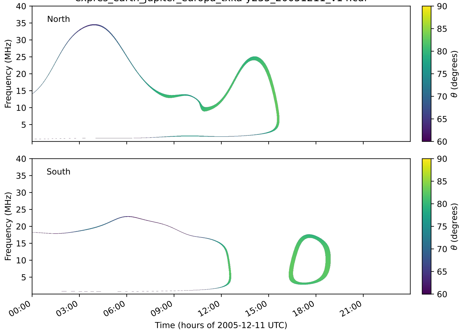
expres_earth_jupiter_europa_txka-y235_20051211_v14.cdf
