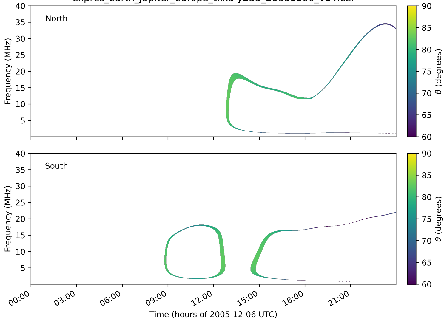
expres_earth_jupiter_europa_txka-y235_20051206_v14.cdf
