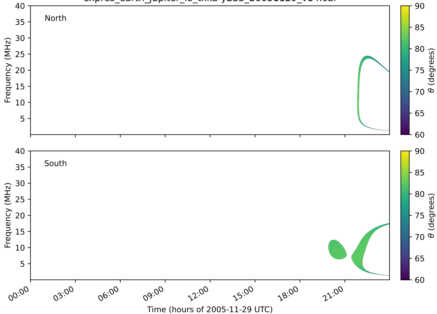
expres_earth_jupiter_io_txka-y235_20051129_v14.cdf
