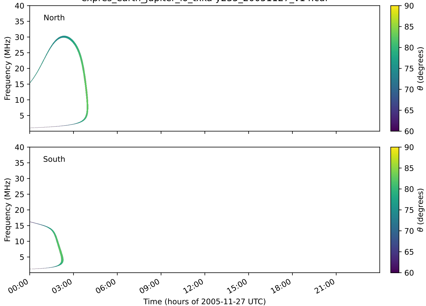
expres_earth_jupiter_io_txka-y235_20051127_v14.cdf
