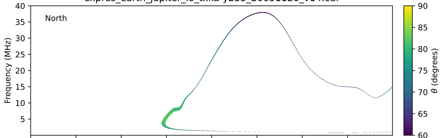
expres_earth_jupiter_io_txka-y235_20051126_v14.cdf
