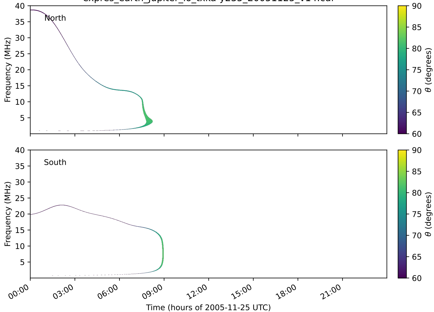
expres_earth_jupiter_io_txka-y235_20051125_v14.cdf
