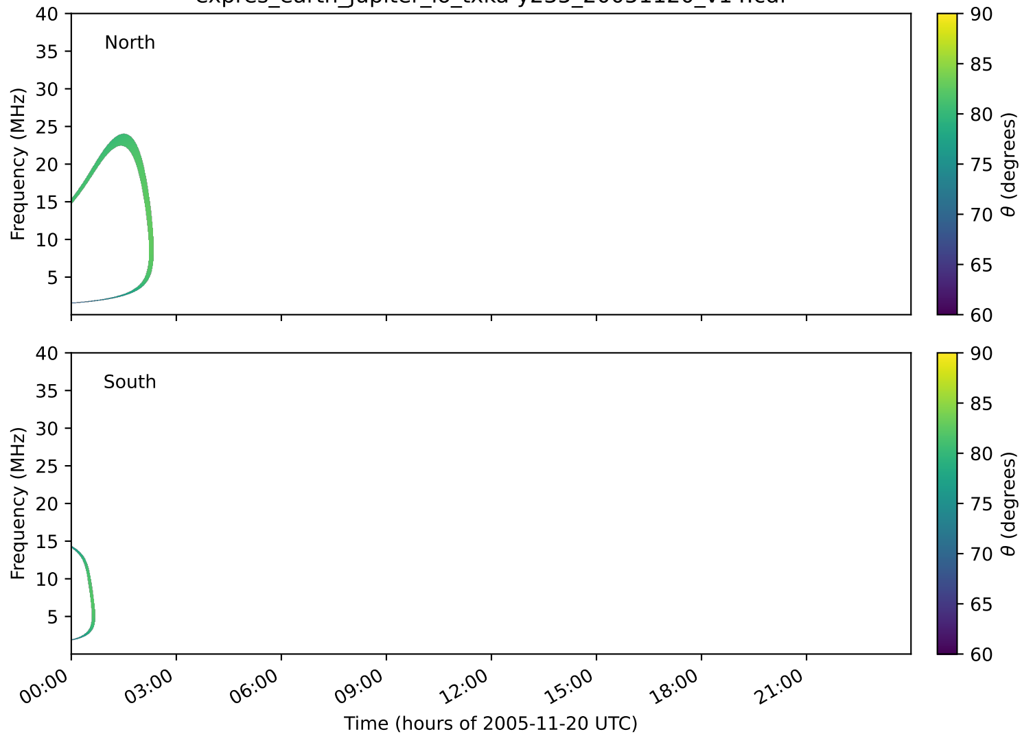
expres_earth_jupiter_io_txka-y235_20051120_v14.cdf
