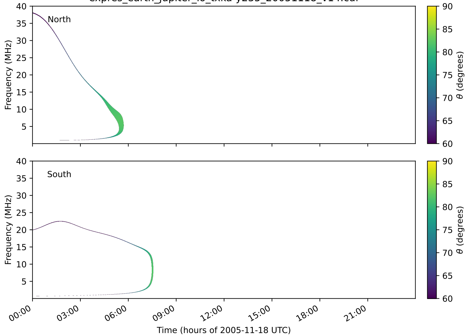
expres_earth_jupiter_io_txka-y235_20051118_v14.cdf
