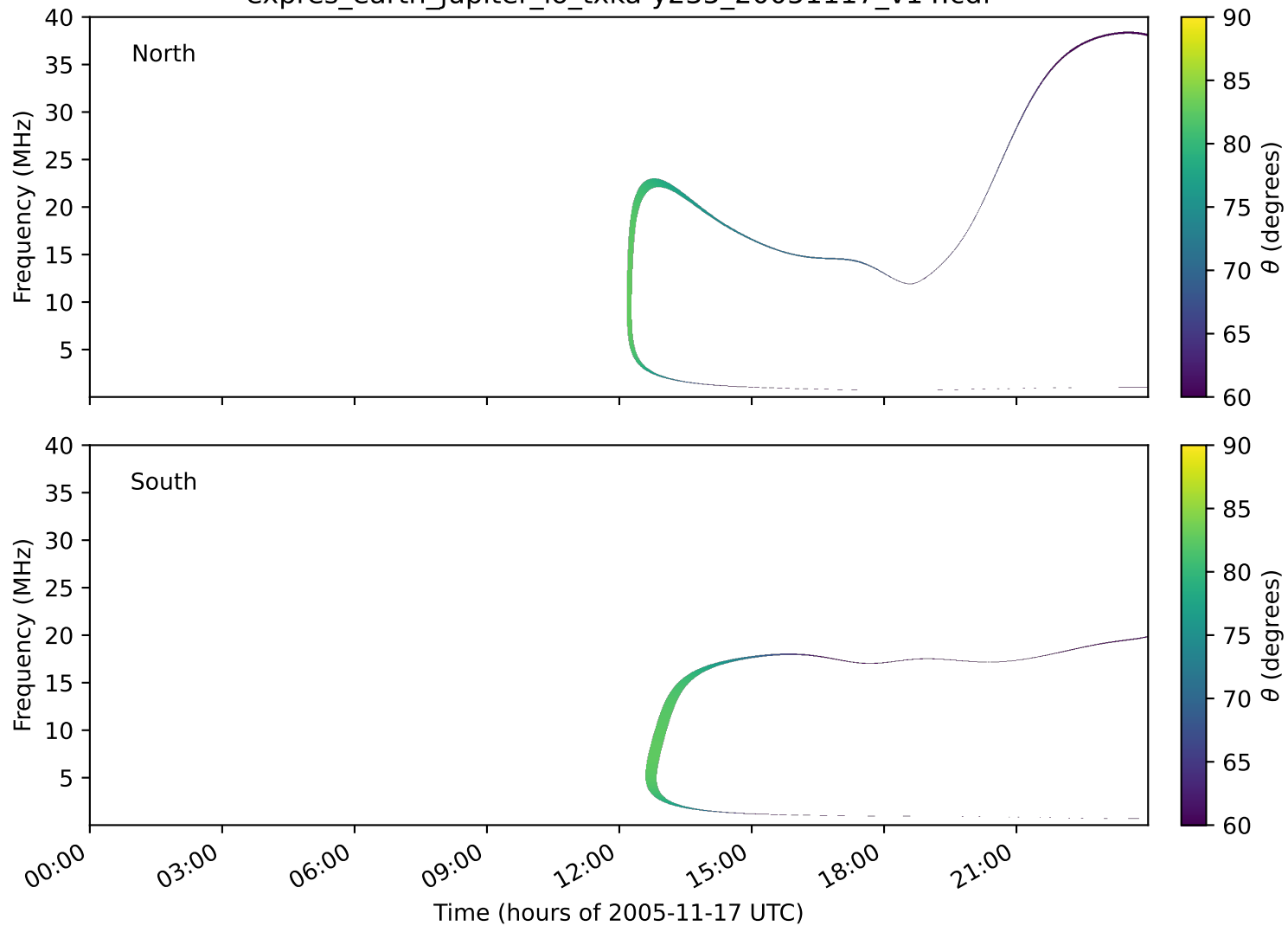
expres_earth_jupiter_io_txka-y235_20051117_v14.cdf
