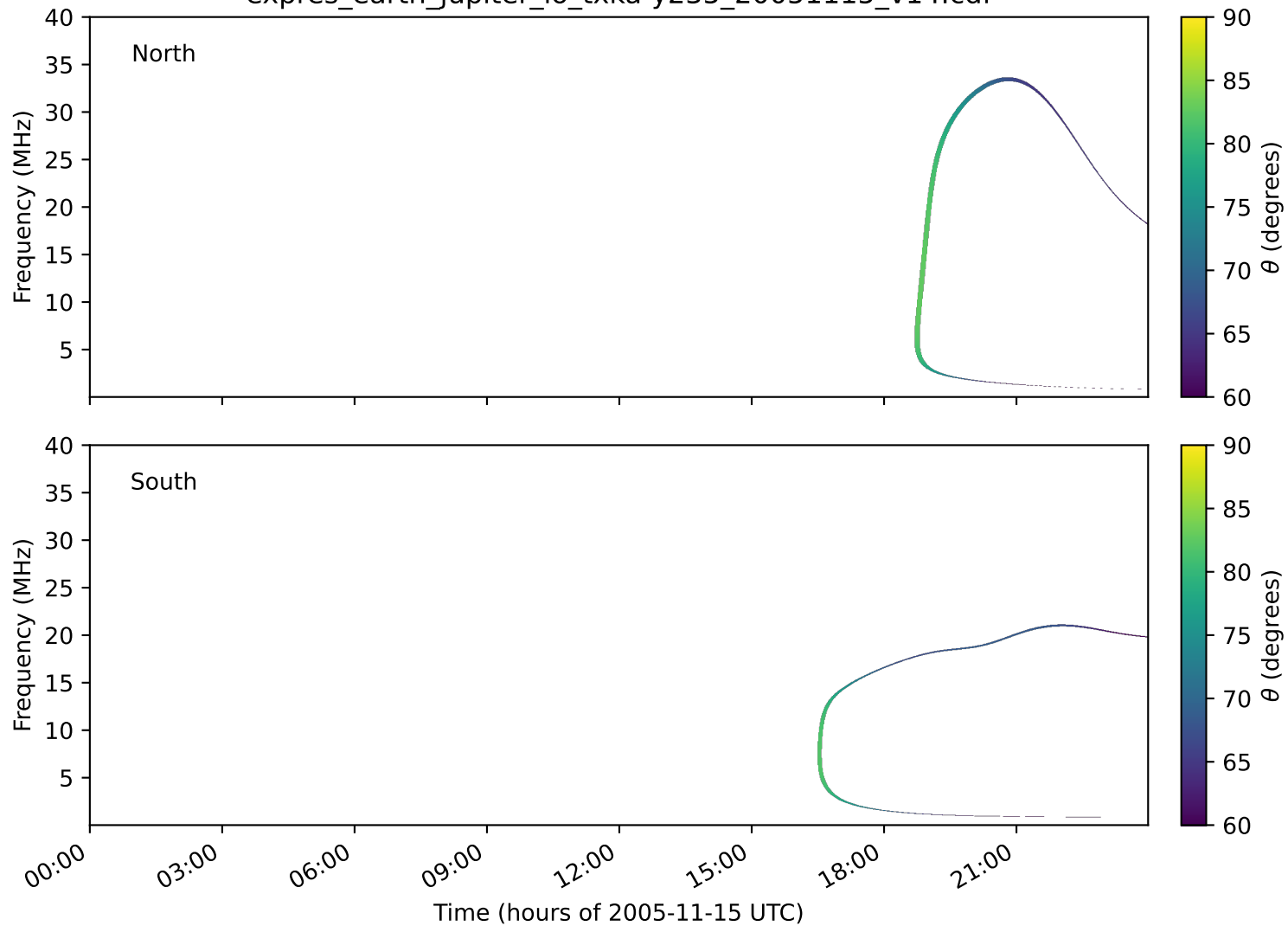
expres_earth_jupiter_io_txka-y235_20051115_v14.cdf
