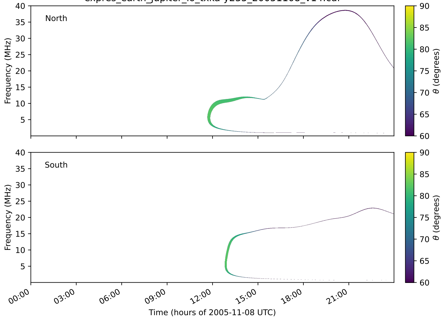
expres_earth_jupiter_io_txka-y235_20051108_v14.cdf
