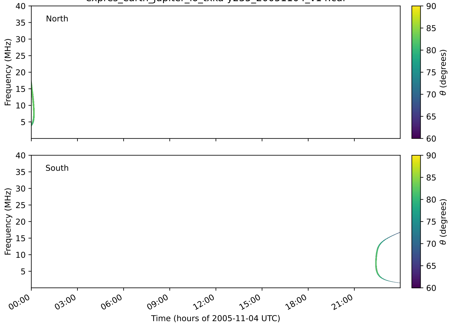
expres_earth_jupiter_io_txka-y235_20051104_v14.cdf
