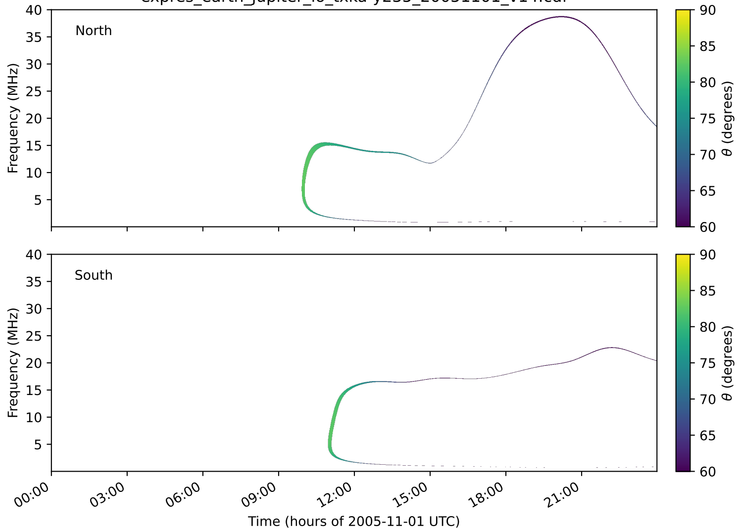
expres_earth_jupiter_io_txka-y235_20051101_v14.cdf
