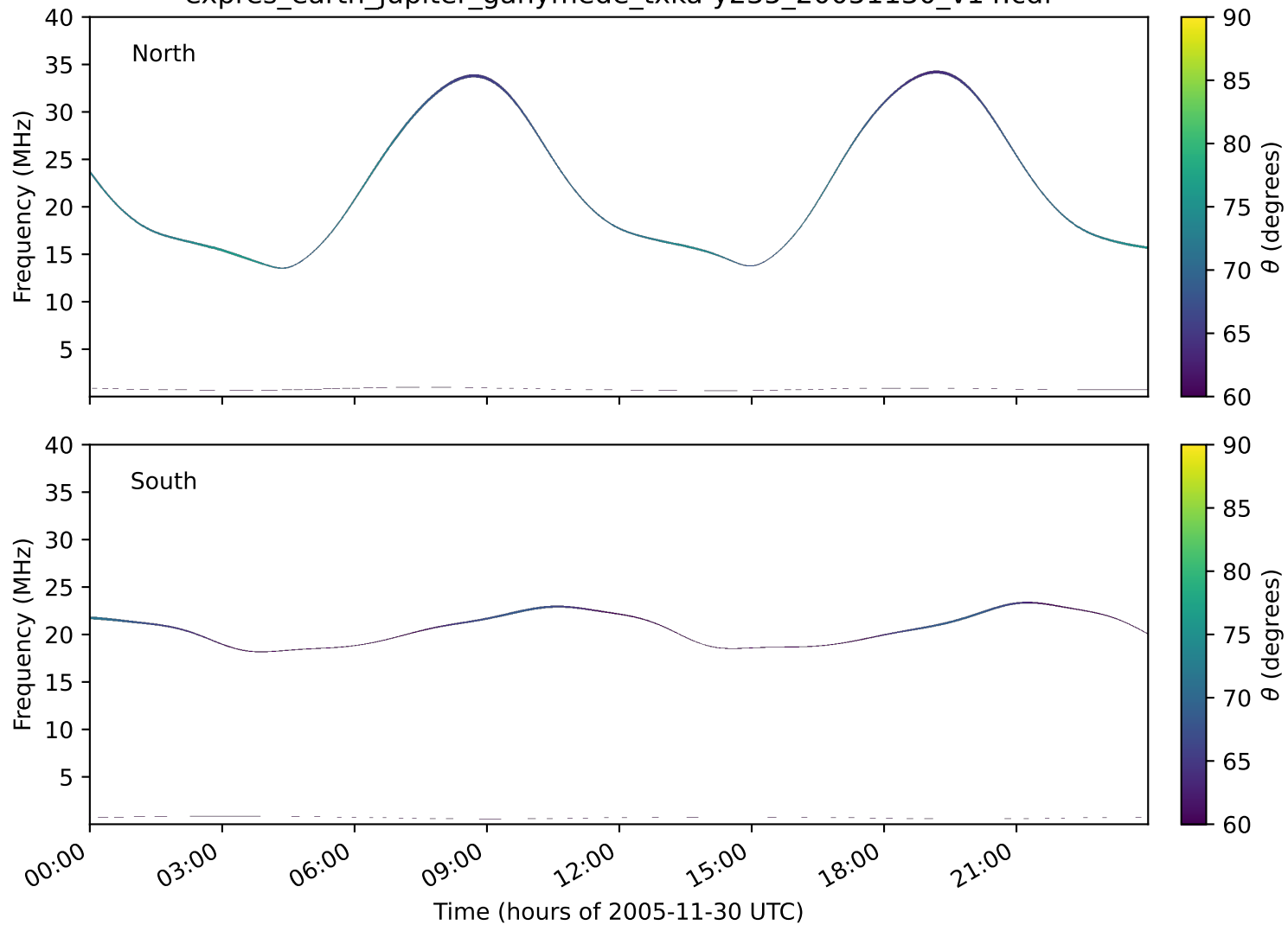
expres_earth_jupiter_ganymede_txka-y235_20051130_v14.cdf
