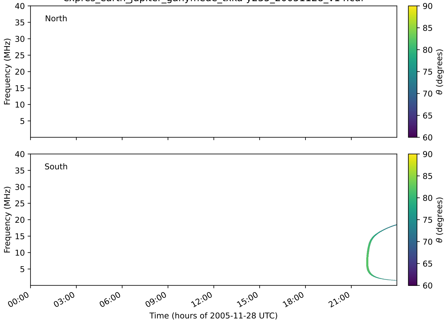
expres_earth_jupiter_ganymede_txka-y235_20051128_v14.cdf
